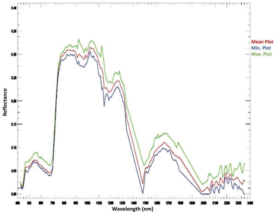
Figure 12: Spectral signature of Poplar in the month of May SPECTRAL SIGNATURE FOR POPLAR (MAY)
