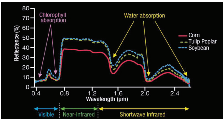
Figure 7: Comparison of signatures of different vegetation on hyperspectral scale
